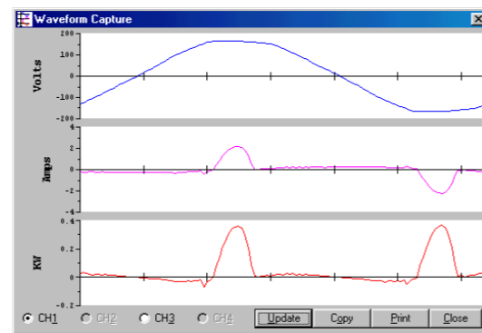
Waveform Capture
